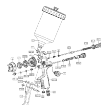
SPARE PARTS EXPLODED VIEW VS 7600 Pag. 328
