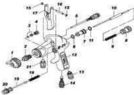
SPARE PARTS EXPLODED VIEW R71 Pag. 342
