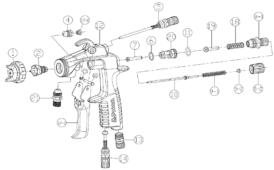
SPARE PARTS EXPLODED VIEW VS820 Pag. 341
