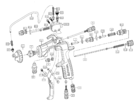
SPARE PARTS EXPLODED VIEW R2102H Pag. 350
