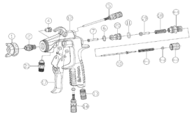
SPARE PARTS EXPLODED VIEW R775 Pag. 339
