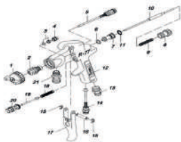
SPARE PARTS EXPLODED VIEW R77 Pag. 343
