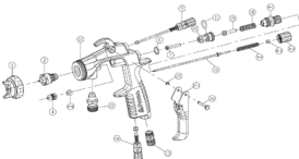
SPARE PARTS EXPLODED VIEW VS810 Pag. 340
