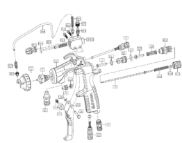
SPARE PARTS EXPLODED VIEW R2101H Pag. 349
