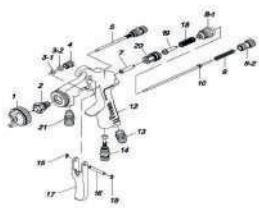
SPARE PARTS EXPLODED VIEW VS503 Pag. 337
