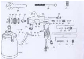
SPARE PARTS EXPLODED VIEW AM6008 Pag. 344
