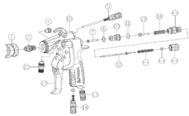
SPARE PARTS EXPLODED VIEW R715 Pag. 338
